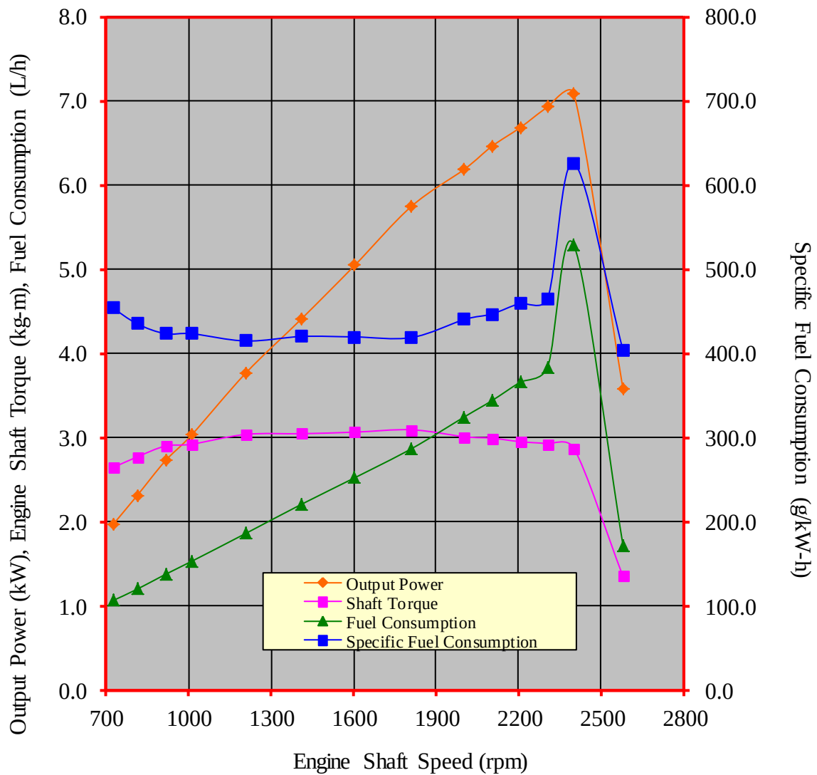
Figure 3. Performance characteristic curves of the GOLDEN BOW JG95 diesel engine
