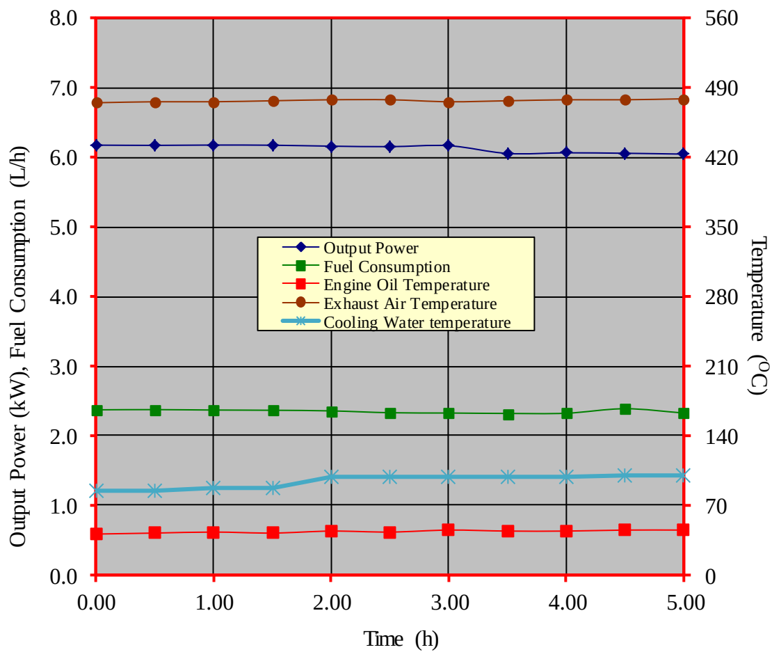
Figure 4. Performance characteristic curves during the continuous running GOLDEN BOW JG95 diesel engine
